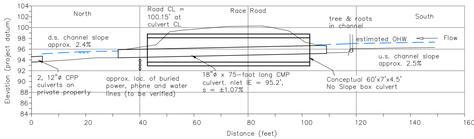
Culvert #1894 Profile View – 2H:1V Distortion
