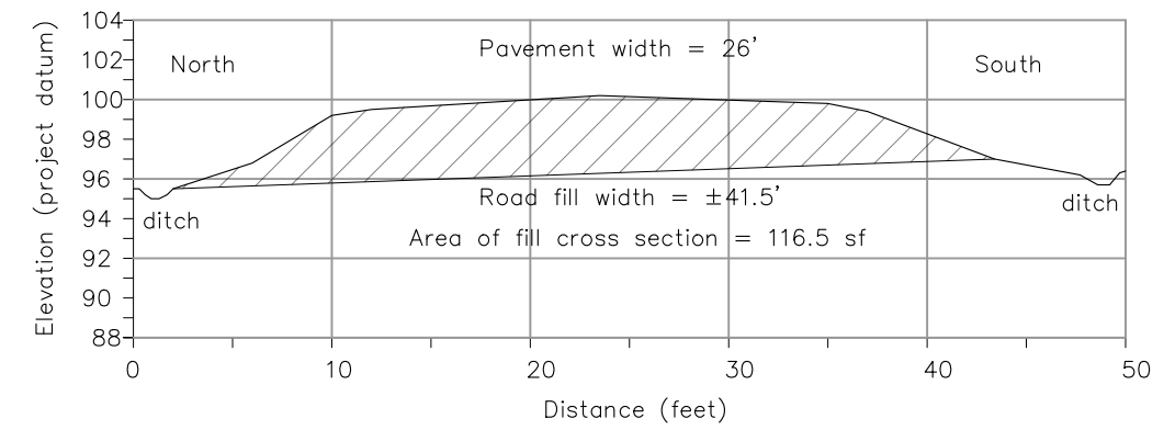
Culvert #1894 Road Prism Cross Section – 1H:1V (10' East of Culvert Crossing)
