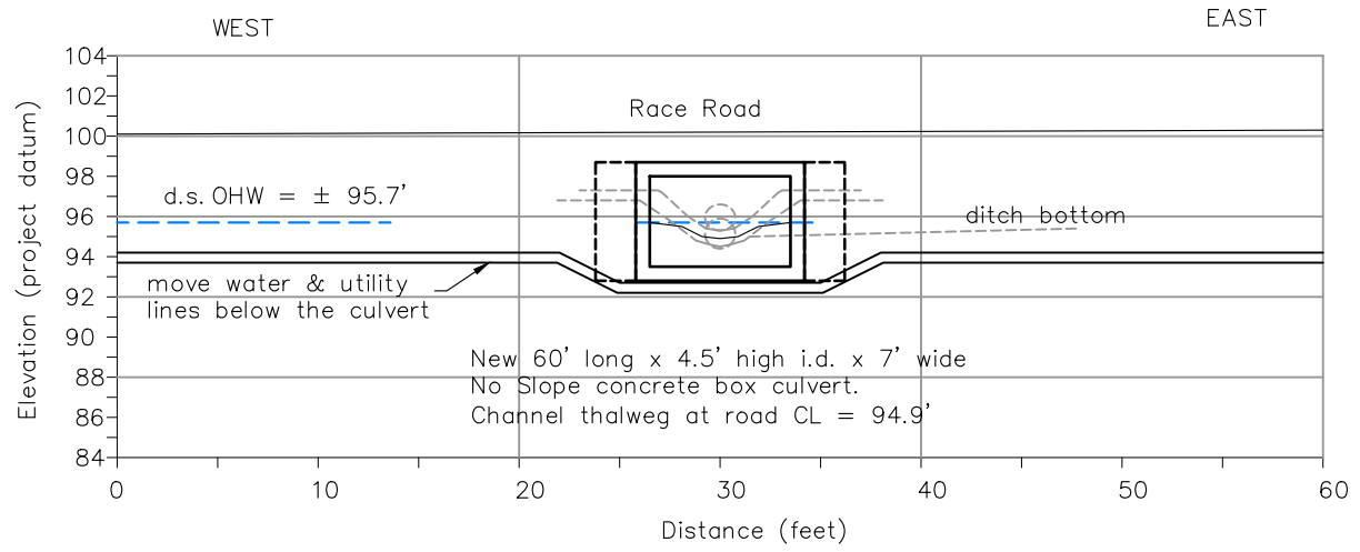
Culvert #1894 Box Culvert Alternative – 1H:1V
