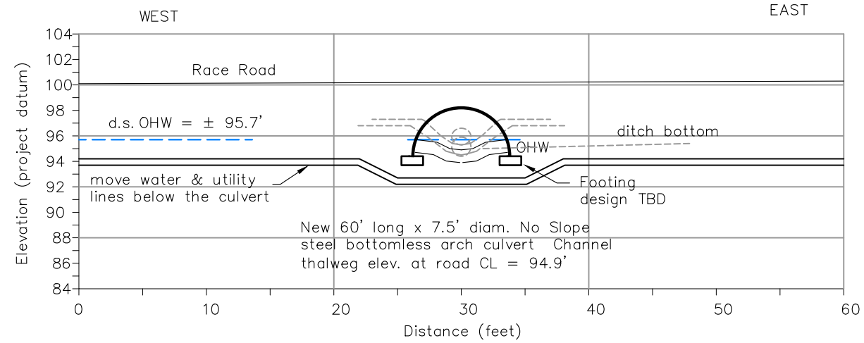
Culvert #1894 Bottomless Arch Culvert Alternative – 1H:1V
