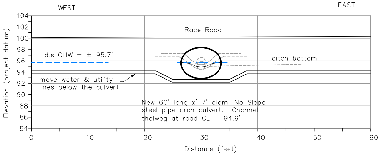
Culvert #1894 Pipe Arch Culvert Alternative – 1H:1V
