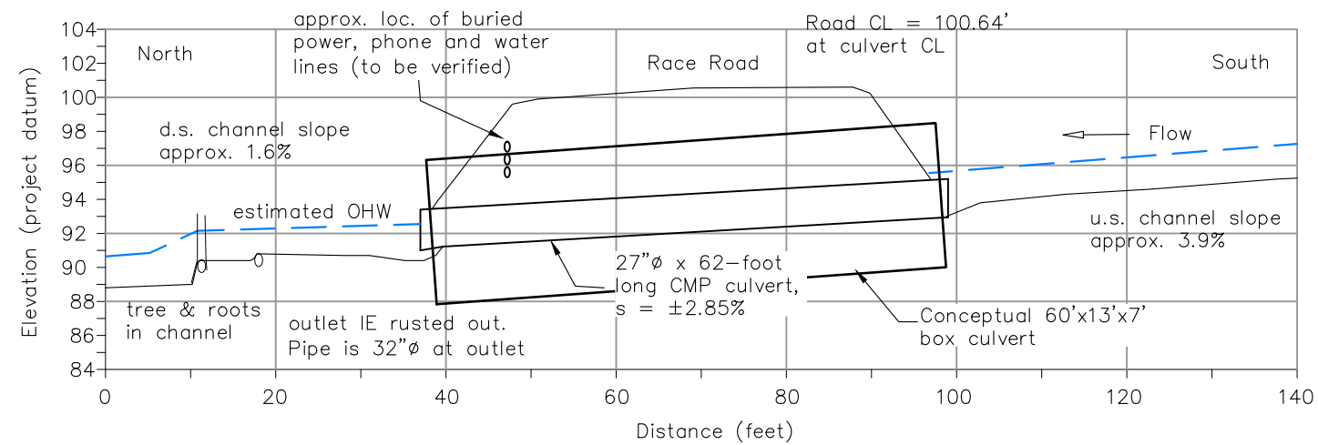
Culvert #1893 Existing Profile View – 2H:1V Distortion
