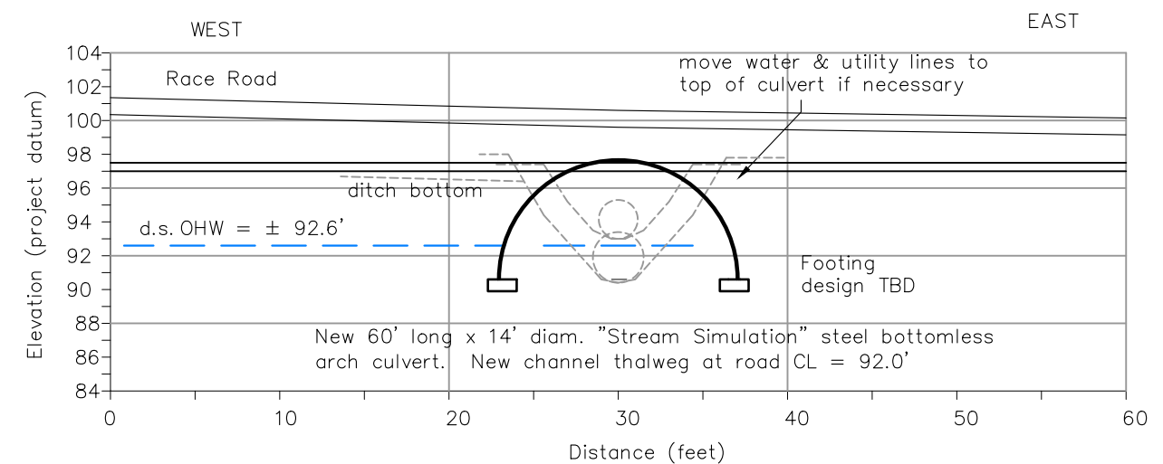
Culvert #1893 Bottomless Arch Culvert Alternative – 1H:1V
