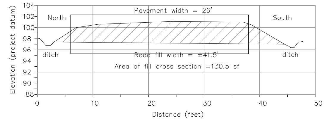
Culvert #1893 Road Prism Cross Section – 1H:1V (10' West of Culvert Crossing)
