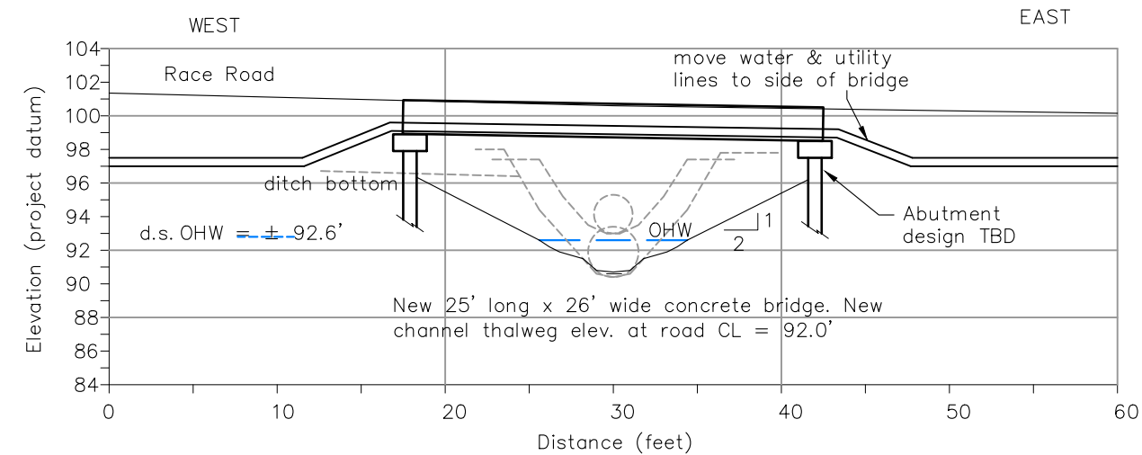
Culvert #1893 Bridge Alternative – 1H:1V
