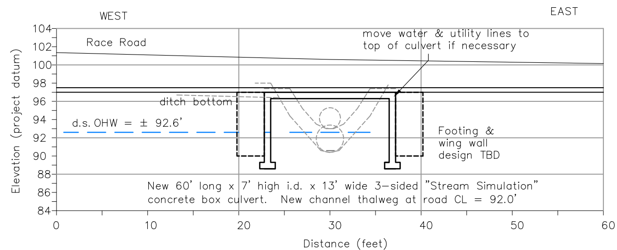
Culvert #1893 Box Culvert Alternative – 1H:1V
