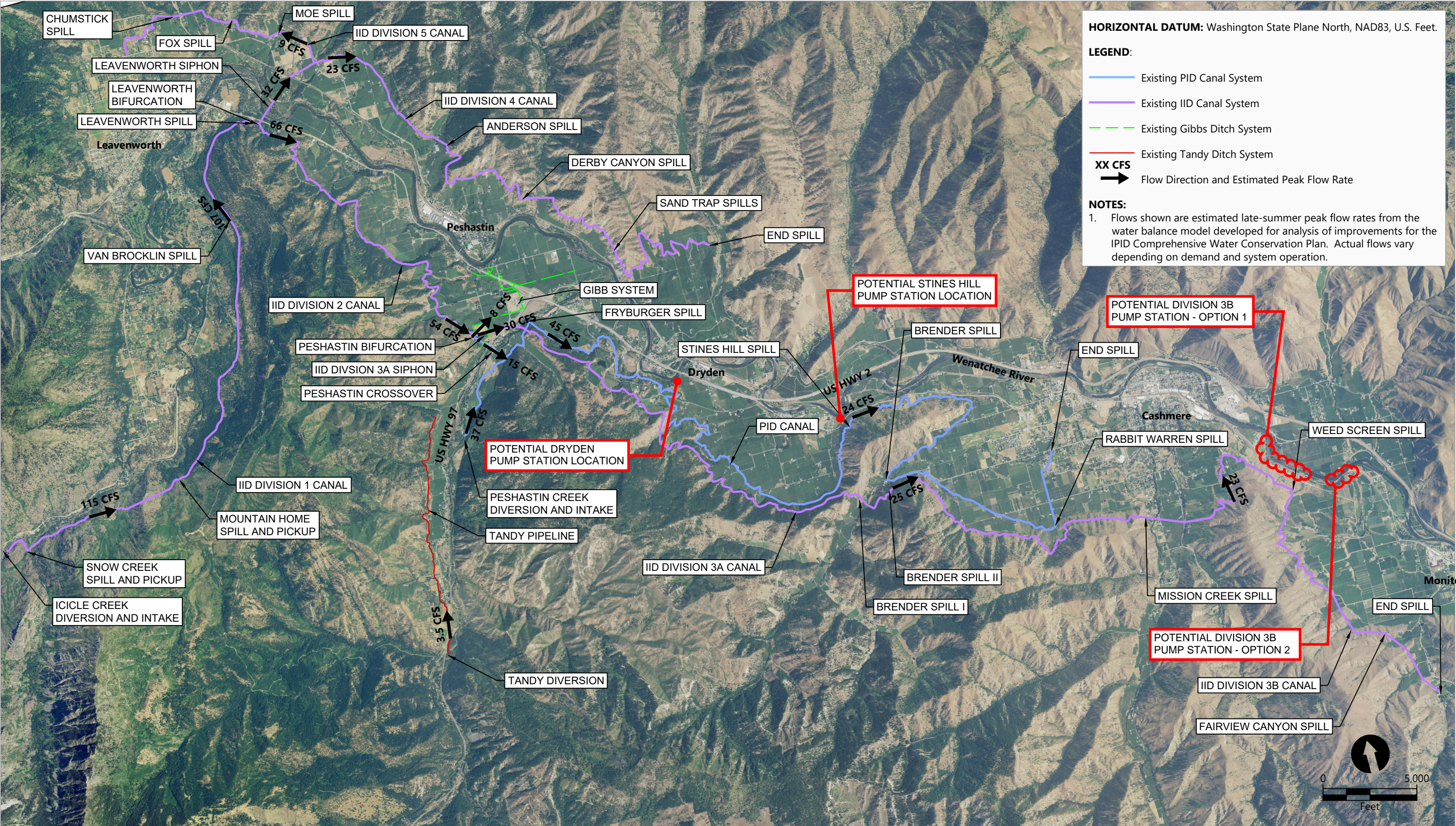
Figure 1 IPID - Existing System and Peak Flows Pump Exchange Expansion Concepts Memorandum Icicle and Peshastin Irrigation Districts
