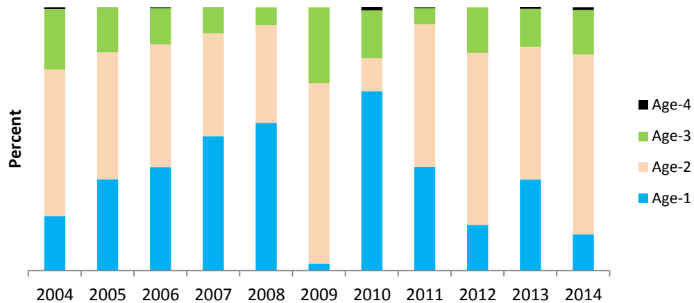
Figure 25. Age structure of emigrants sampled during spring out-migrations, 2004-2014. Reproduced from Crawford et al. (2015).
